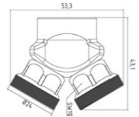
2-YV Y-Stück 50° Y-piece 50°
